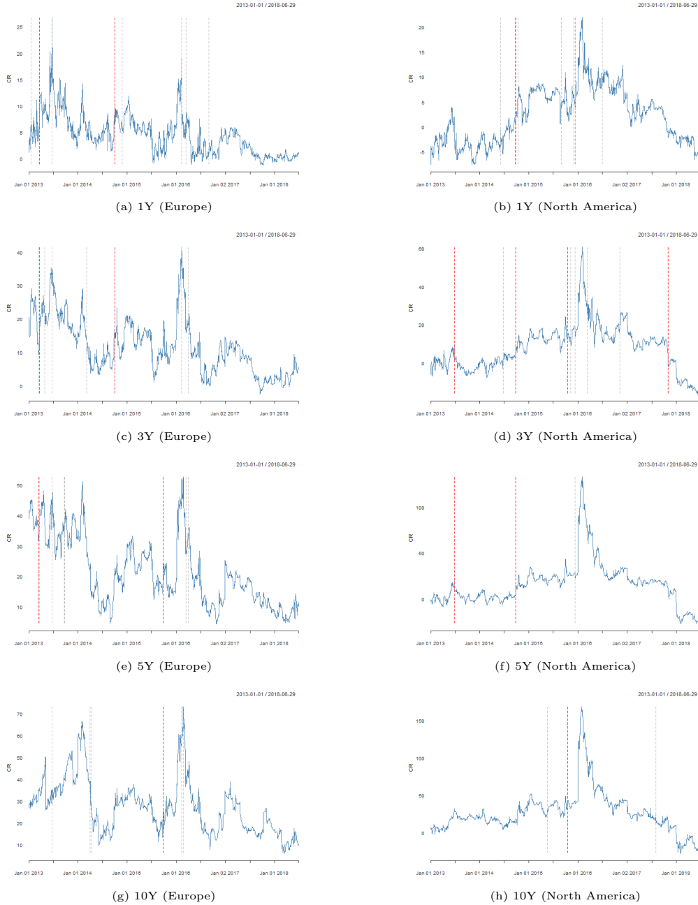
Figure 12: Evolution of CR factor over time for maturities 1Y (top), 3Y (top center), 5Y (bottom center) and 10Y (bottom) for Europe (left) and North America (right). The vertical solid lines indicate events where both the news index and the CR jointly deviate by a factor of 1.5 standard deviations from their respective means.
