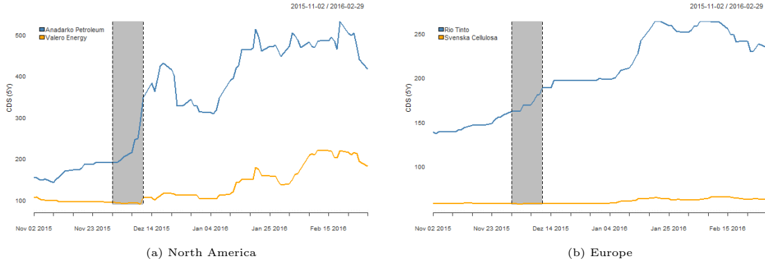
Figure 15: Evolution of the 5Y-CDS spreads of Anadarko Petroleum (blue) and Valero Energy (orange) on the left diagram, and Rio Tinto (blue) and Svenska Cellulosa (orange) on the right diagram. The time period spans from 02 November 2015 to 29 February 2016. The gray-shaded area indicates the time period of COP21 (30th Nov 2015 – 12th Dec 2015).
