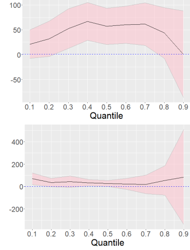
Figure 8: Left panels: Coefficient estimates of the ETS share QR model as well as the respective mean (OLS) regression model for 5-year CDS spread returns in Europe (top) and North America (bottom), respectively. The sample comprises data for 119 European firms and 164 North American firms from 2013/01/01 to 2019/12/31 in daily frequency. Estimates and standard errors (in brackets) are reported for the 1st, 5th, and 9th decile, and the mean. All estimates are scaled by factor 1000. Right panels: Graphic visualization of the \Delta CR \times ETS(Yes) \times ETS share QR estimates for all nine deciles. The pink-shaded area indicates the 95% confidence interval. The blue dashed line represents the respective value of the OLS estimate.
