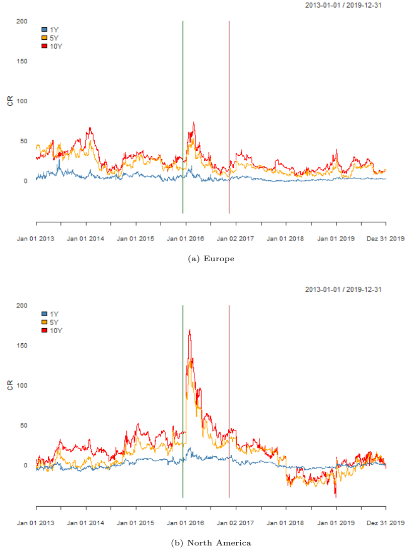
Figure 2: Evolution of the CR factor over time for maturities 1Y (blue), 5Y (orange) and 10Y (red) for Europe (top) and North America (bottom). The vertical solid lines indicate the timing of the Paris Agreement (dark green) and Trump election (brown), respectively.
