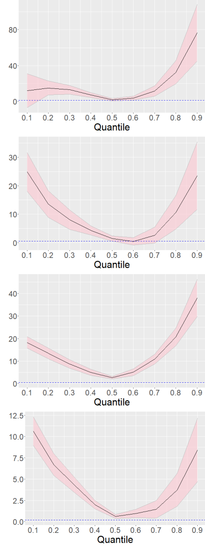
Figure 5: Left panels: Coefficient estimates of the base panel QR model as well as the mean (OLS) regression model for 1-year (top), 3-year (upper center), 5-year (lower center), and 10-year (bottom) CDS spread returns. The sample comprises data for 164 North American firms from 2013/01/01 to 2019/12/31 in daily frequency. Estimates and standard errors (in brackets) are reported for the 1st, 5th, and 9th decile, and the mean. All estimates are scaled by factor 1000. Right panels: Graphic visualization of the \Delta CR QR estimates for all nine deciles. The pink-shaded area indicates the 95% confidence interval. The blue dashed line represents the respective value of the OLS estimate.
