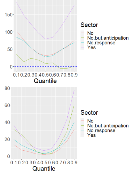
Figure 7: Left panels: Coefficient estimates of the ETS QR model as well as the respective mean (OLS) regression model for 5-year CDS spread returns in Europe (top) and North America (bottom). The sample comprises data for 119 European firms and 164 North American firms from 2013/01/01 to 2019/12/31 in daily frequency. Estimates and standard errors (in brackets) are reported for the 1st, 5th, and 9th decile, and the mean. All estimates are scaled by factor 1000. Right panels: Graphic visualization of all ETS interaction estimates for all nine deciles. The blue dashed line represents the zero line.
