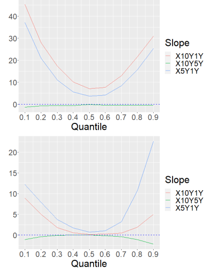
Figure 11: Left panels: Coefficient estimates of the term structure QR model as well as the respective mean (OLS) regression model for 5Y-1Y, 10Y-5Y, and 10Y-1Y CDS spread slope changes in Europe (top) and North America (bottom). The sample comprises data for 119 European firms and 164 North American firms from 2013/01/01 to 2019/12/31 in daily frequency. Estimates and standard errors (in brackets) are reported for the 1st, 5th, and 9th decile, and the mean. All estimates are scaled by factor 1000. Right panels: Graphic visualization of all three slope estimates for all nine deciles. The blue dashed line represents the zero line.
