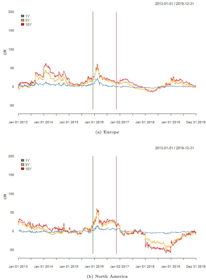
Figure 13: Evolution of the CR factor (controlled for sectors) over time for maturities 1Y (blue), 5Y (orange) and 10Y (red) for Europe (top) and North America (bottom). The vertical solid lines indicate the timing of the Paris Agreement (dark green) and Trump election (brown), respectively.
